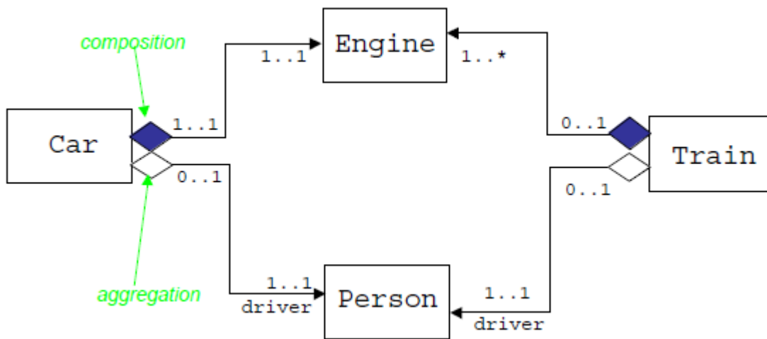
Figure: Composition and Aggregation Example
