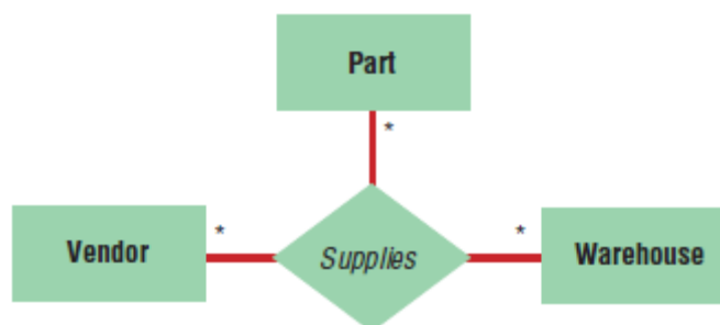
Figure: Ternary Associations
