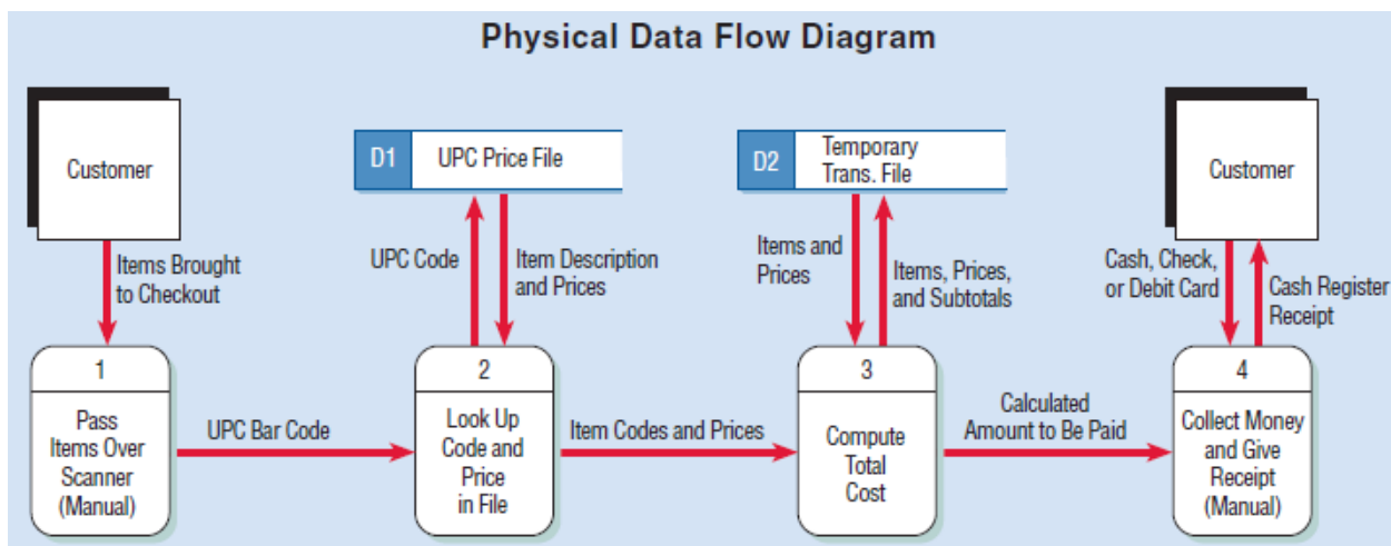
Figure: The physical data flow diagram (below) shows certain details not found on the logical data flow diagram (above).
