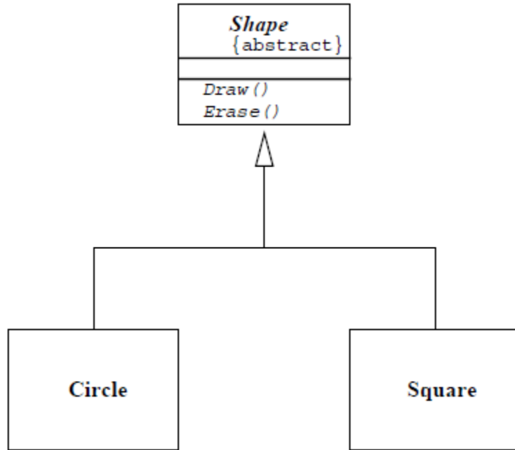
Figure: Inheritance Example
