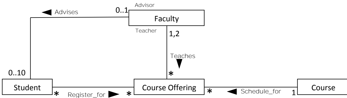
Figure: n-ary Associations
