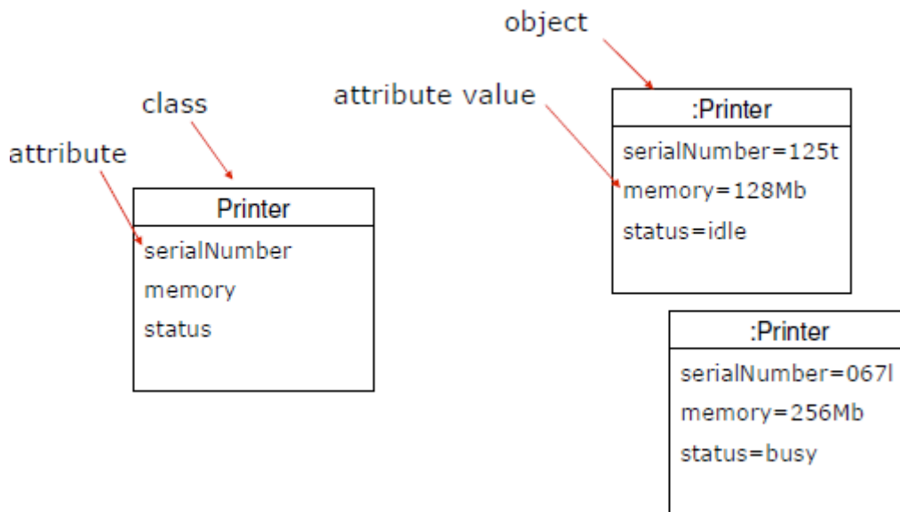
Figure: Attribute Examples
