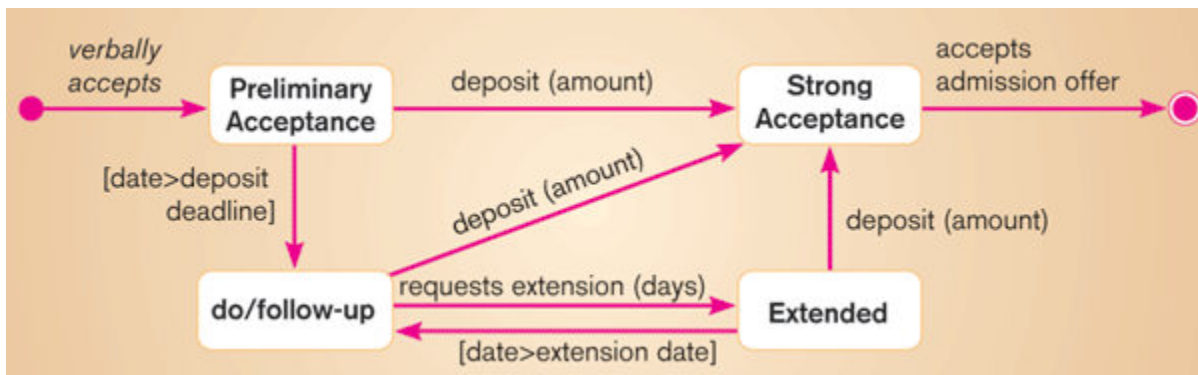
Figure: Nested state diagram for the accepts admission offer event
