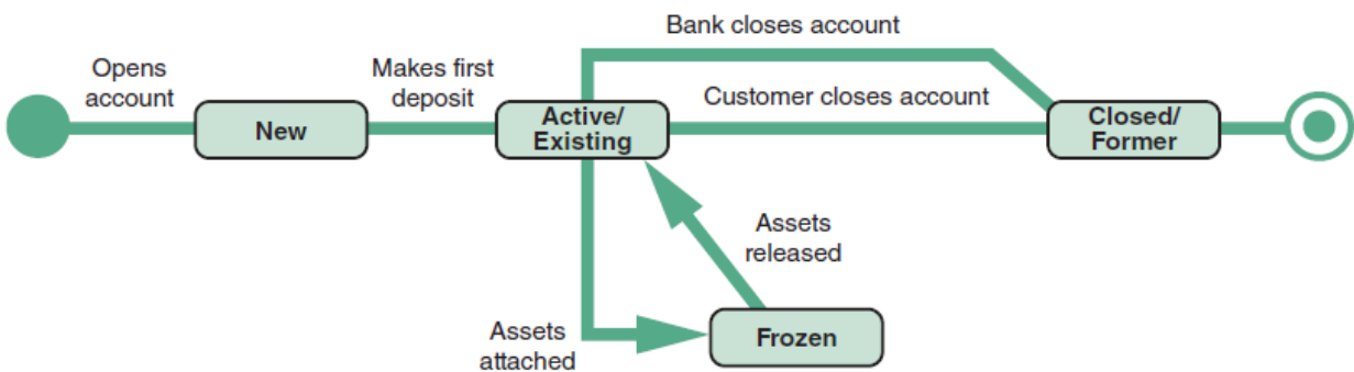
Figure: An example of a state transition diagram for a bank account.
