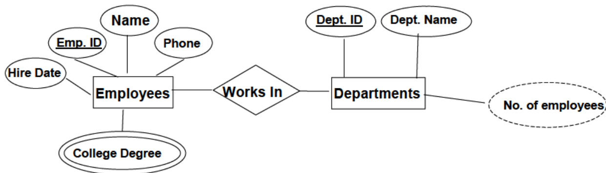
Figure: Example of an ERD
