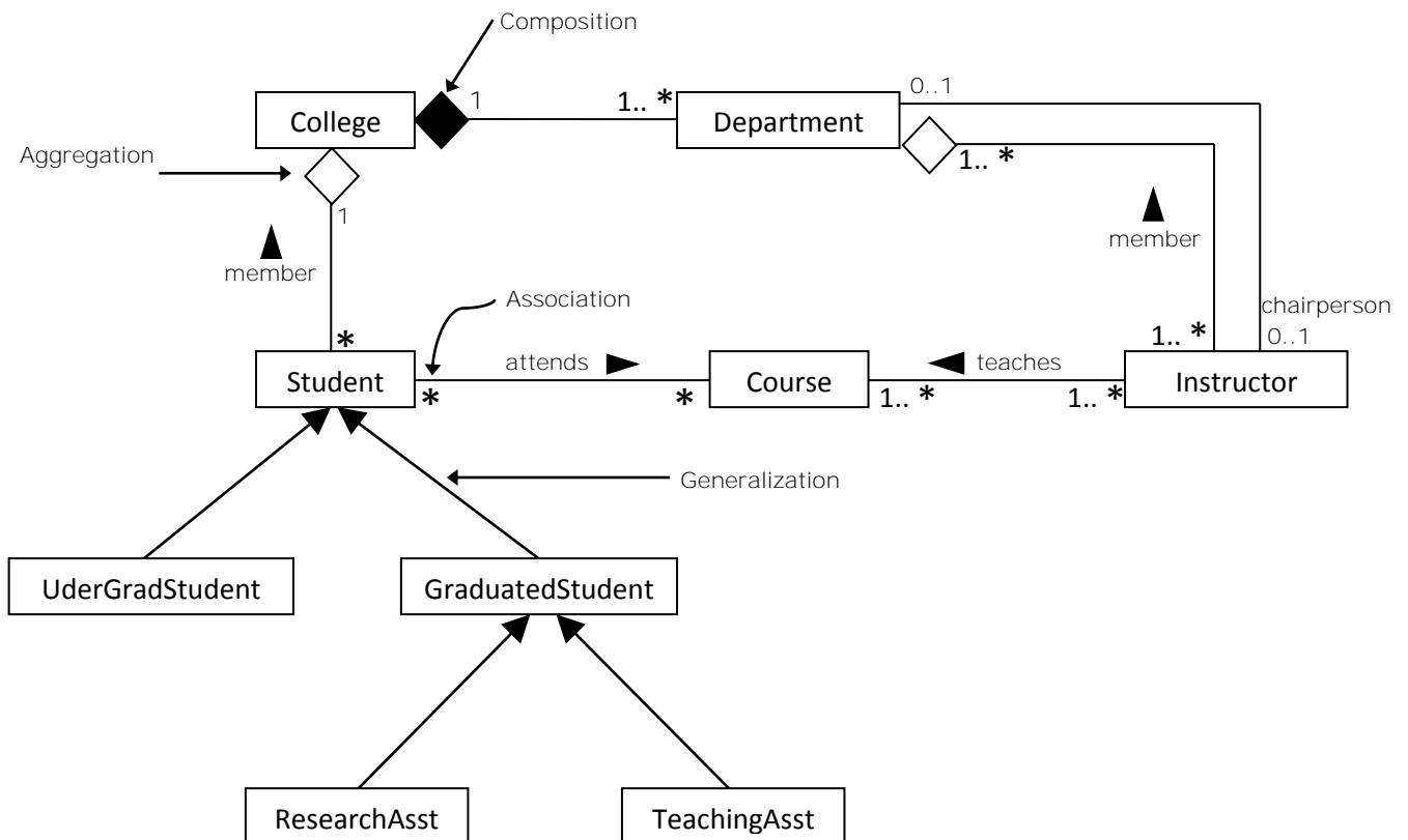
Figure: Class Diagram for a College System.
