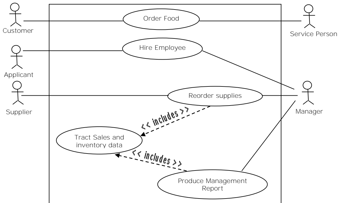
Figure: Use-Case diagram for a Burger's System
