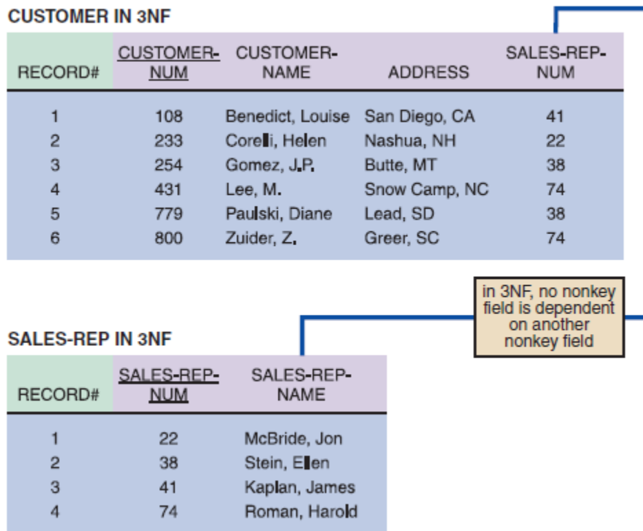
Figure: When the CUSTOMER table is transformed from 2NF to 3NF, the result is two tables: CUSTOMER and SALES-REP
