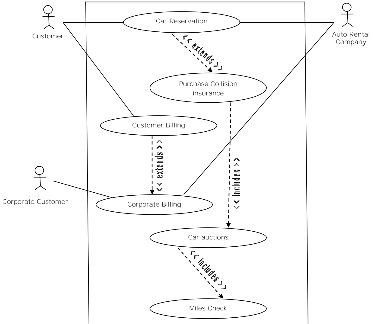
Figure: Use Case diagram: A diagram that depicts the Use Cases and action for a system
