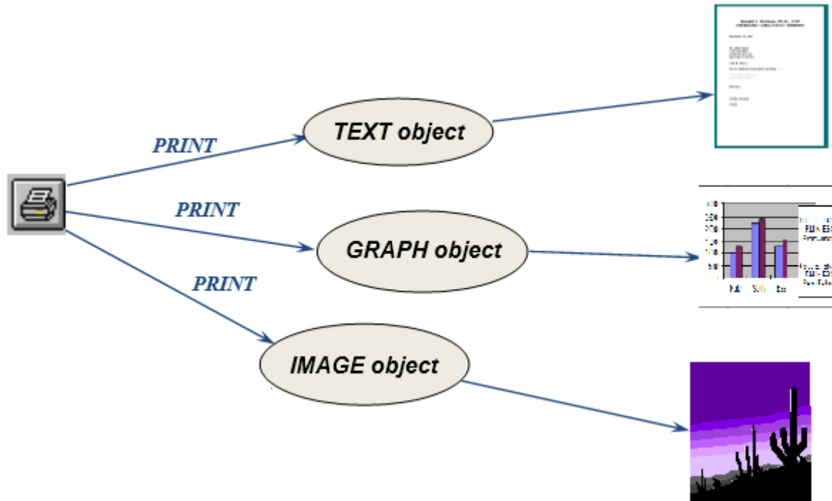
Figure: Polymorphism Example
