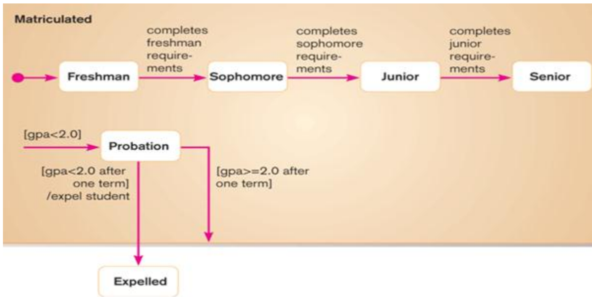
Figure: A nested state diagram for Matriculated state of Student object
