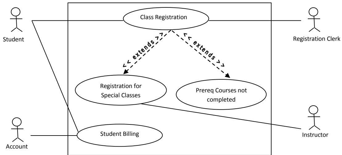
Figure: Use-Case diagram for a University Registration System
