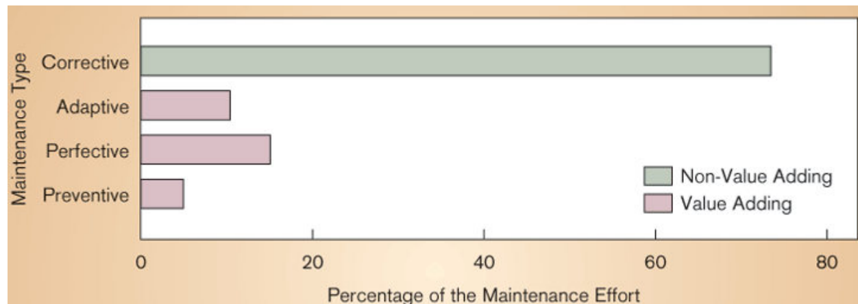
Figure: Maintenance Types and their Corresponding Efforts
