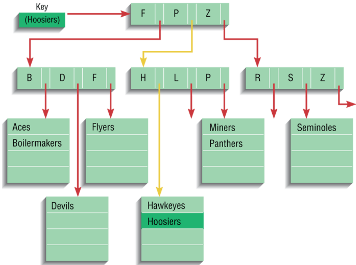
Figure: Indexed Sequential Organization
