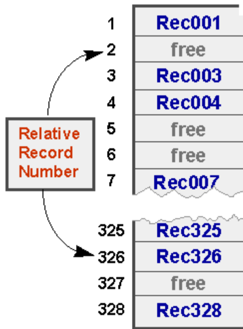
Figure: Direct-Access Organization
