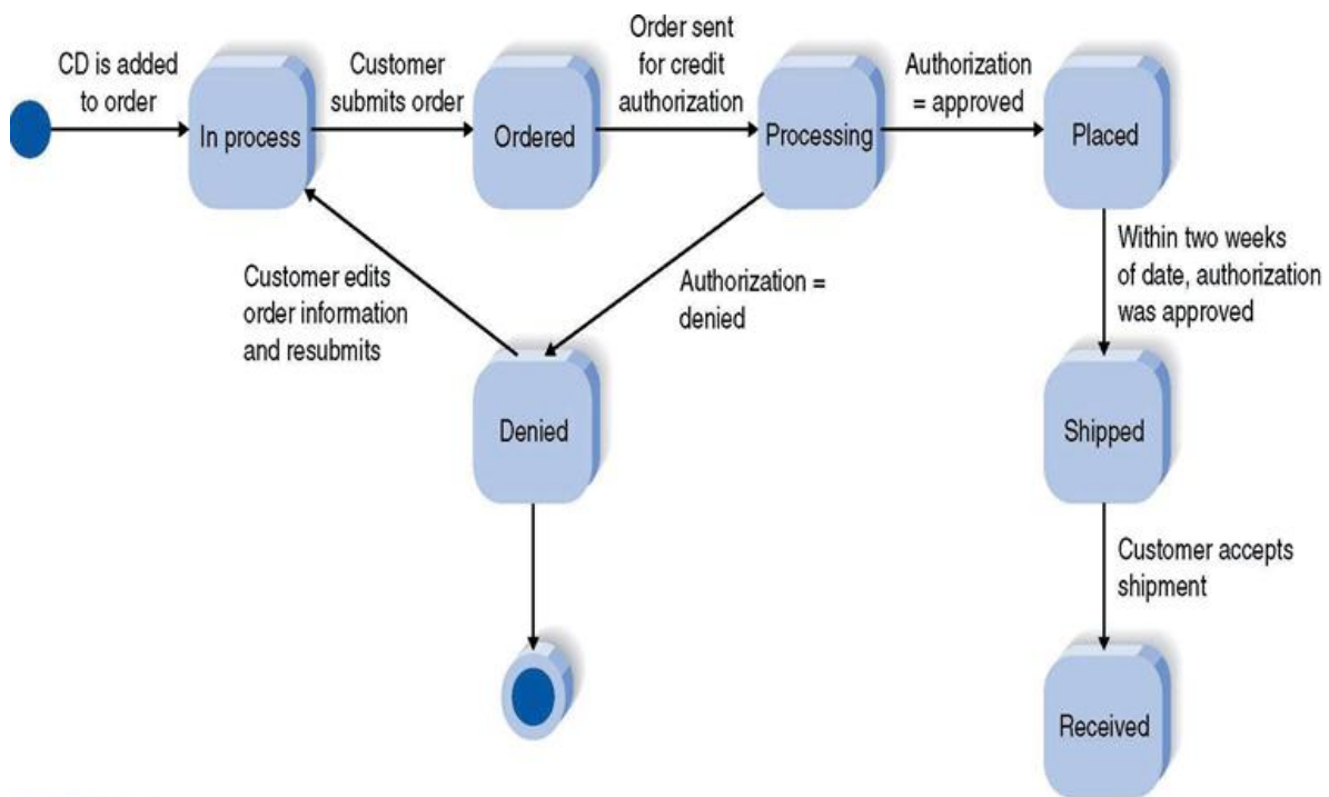
Figure: State diagram for ordering CDs
