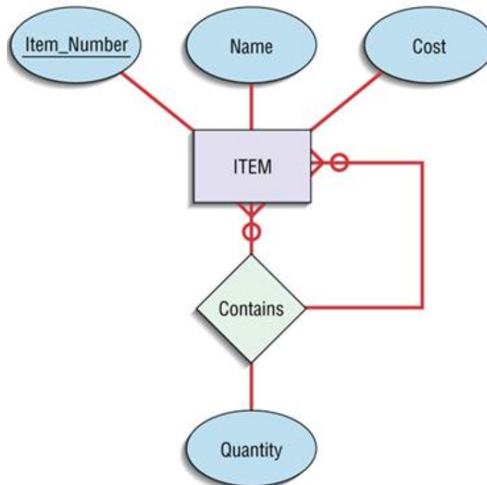
Figure: Two unary relations – Bill-of-materials structure (M:N)
