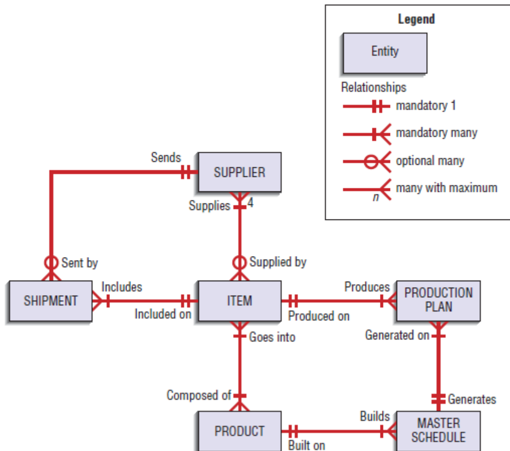
Figure: Sample conceptual data model diagrams: Standard E-R notation.
