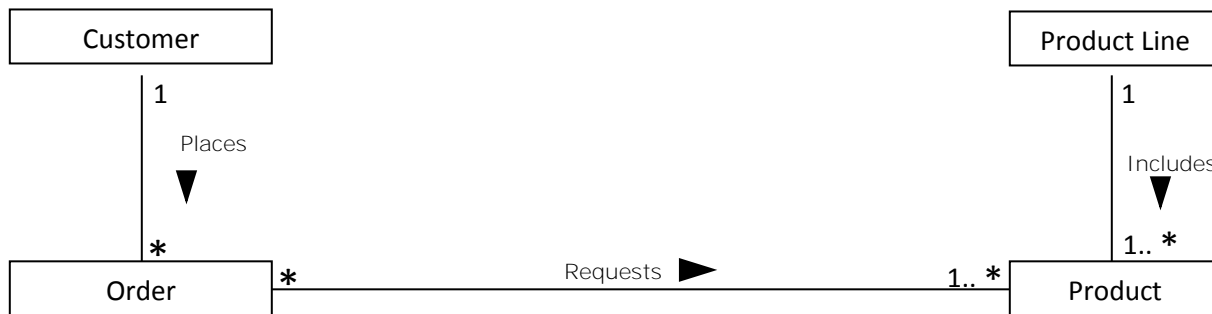
Figure: Class diagram for "Customer Order"
