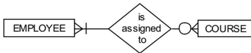
One optional, One mandatory cardinality
