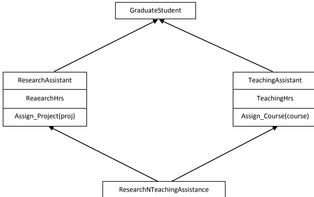
Figure: Multiple Inheritance
