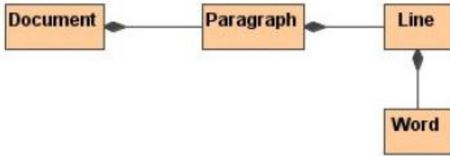
Figure: Composition Example
