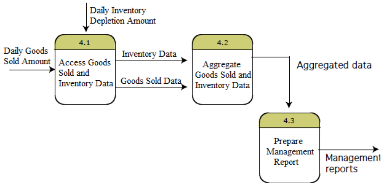
Figure: Level-1 Diagram Showing the Decomposition of Process 4.0 from the Level-0 Diagram
