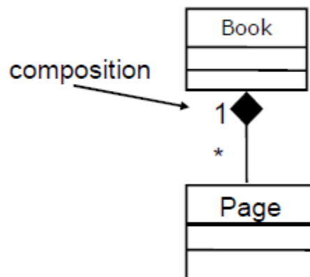
Figure: Composition Example
