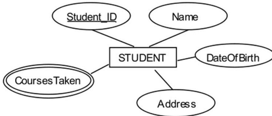
Figure: Entity, Attributes, and Multivalued Attributes
