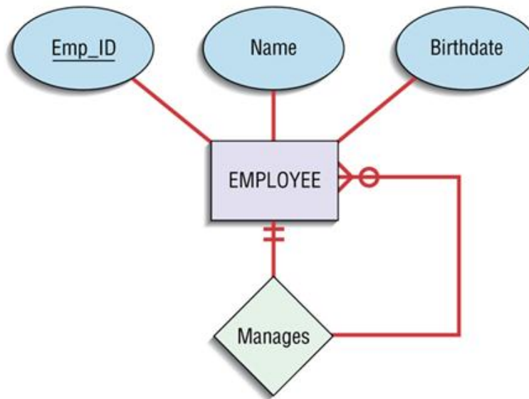
Figure: Two unary relations – EMPLOYEE with Manages relationship (1:N)
