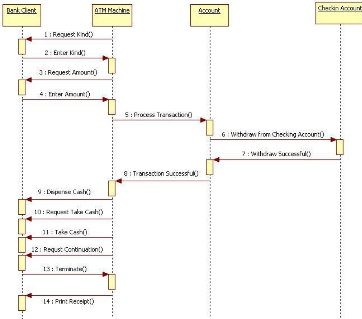
Figure: An Example of Sequence Diagram for ATM
