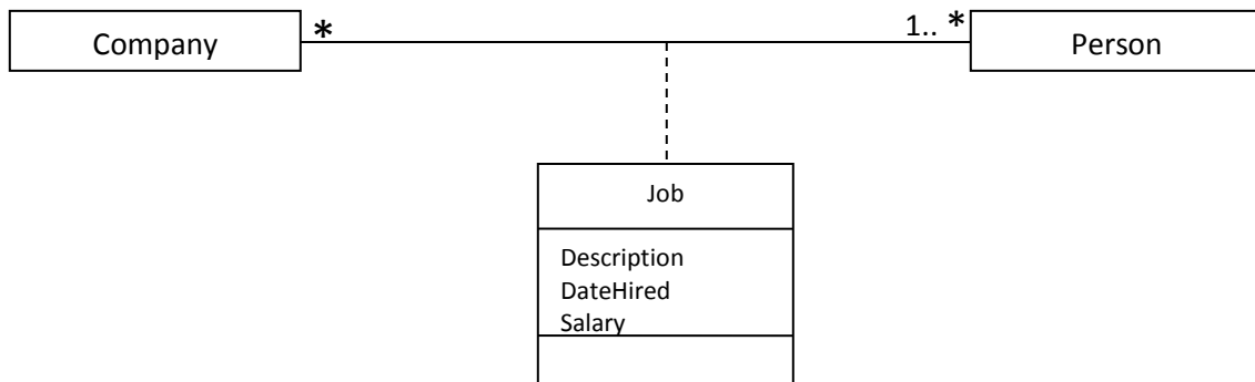
Figure: Class diagram showing an association class “Job”
