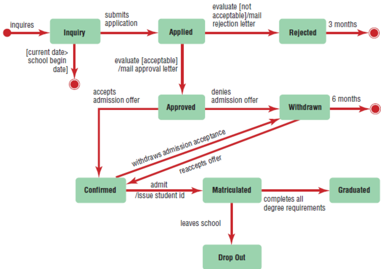
Figure: State diagram for the Student object.
