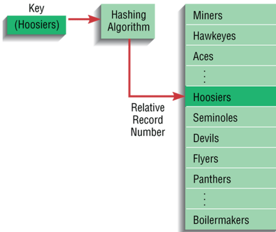
Figure: Hashed File Organization
