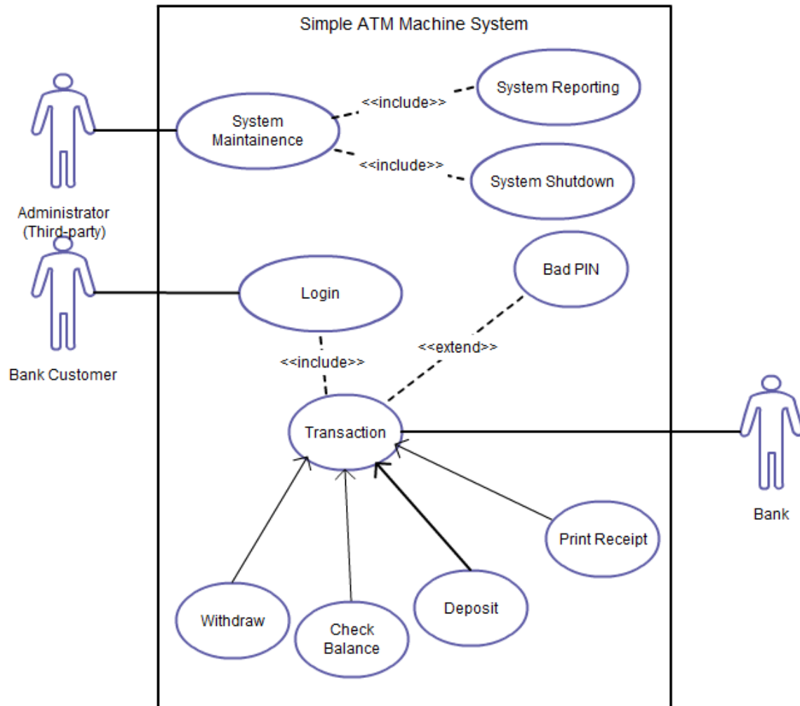
Figure: Use case diagram of ATM Machine System
