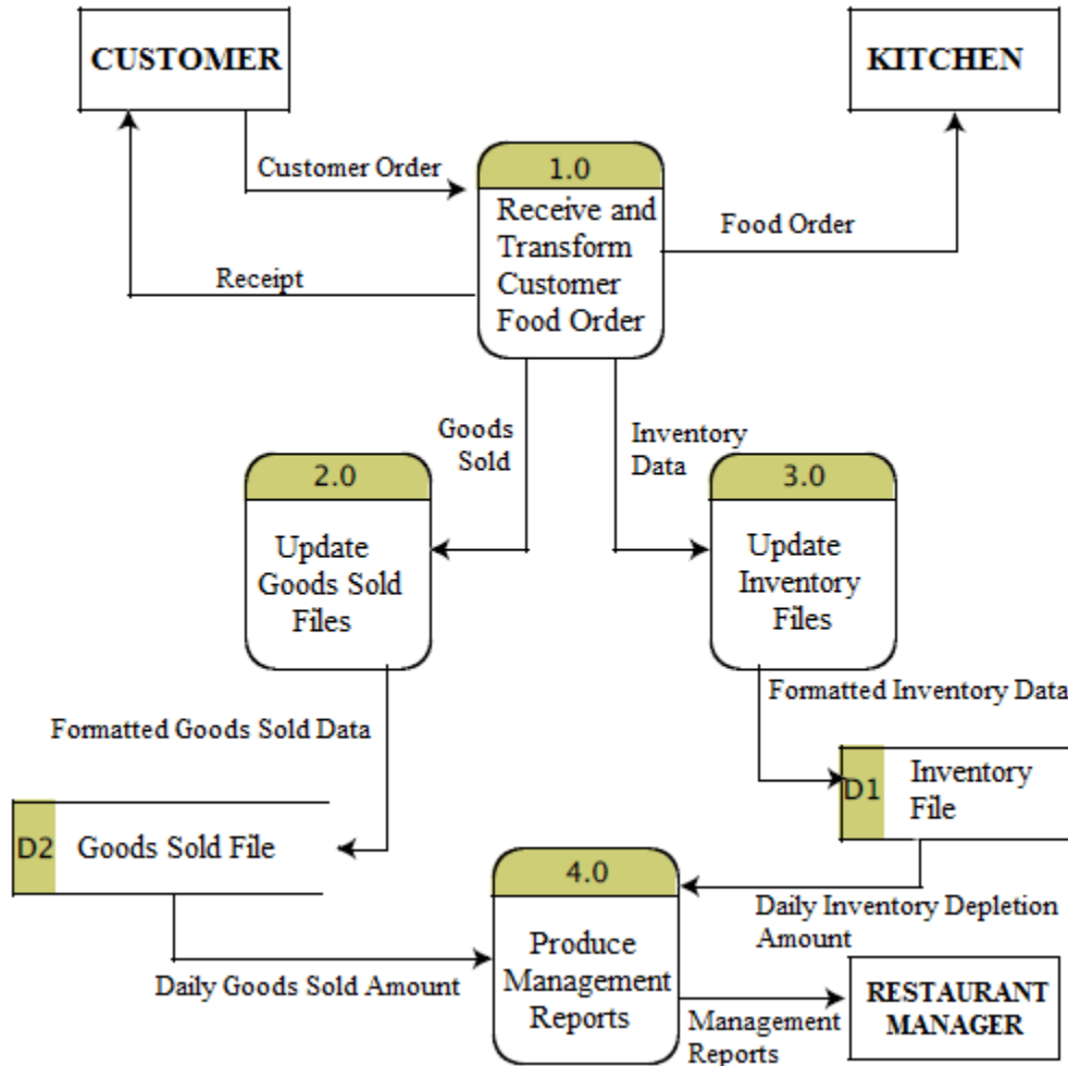
Figure: Level-0 DFD of Food Ordering System
