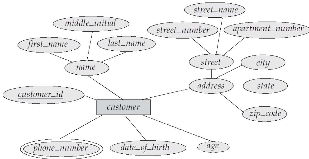
Figure: Composite Attributes, Derived Attributes and Multi-valued Attributes
