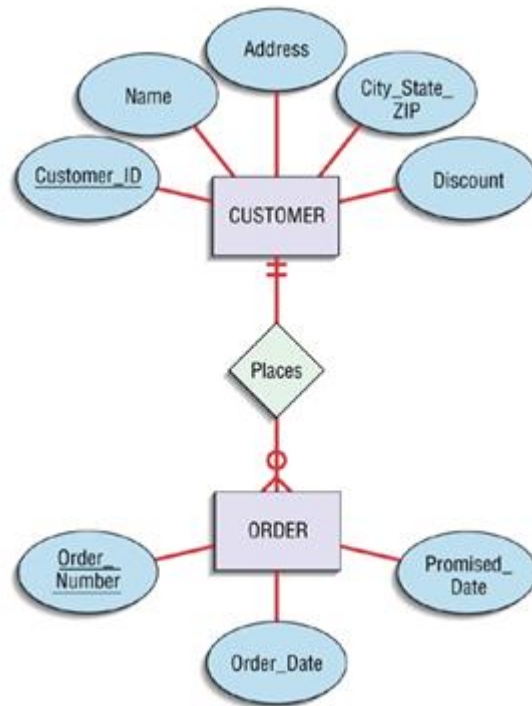
Figure: Representing a 1:N relationship – ER Diagram
