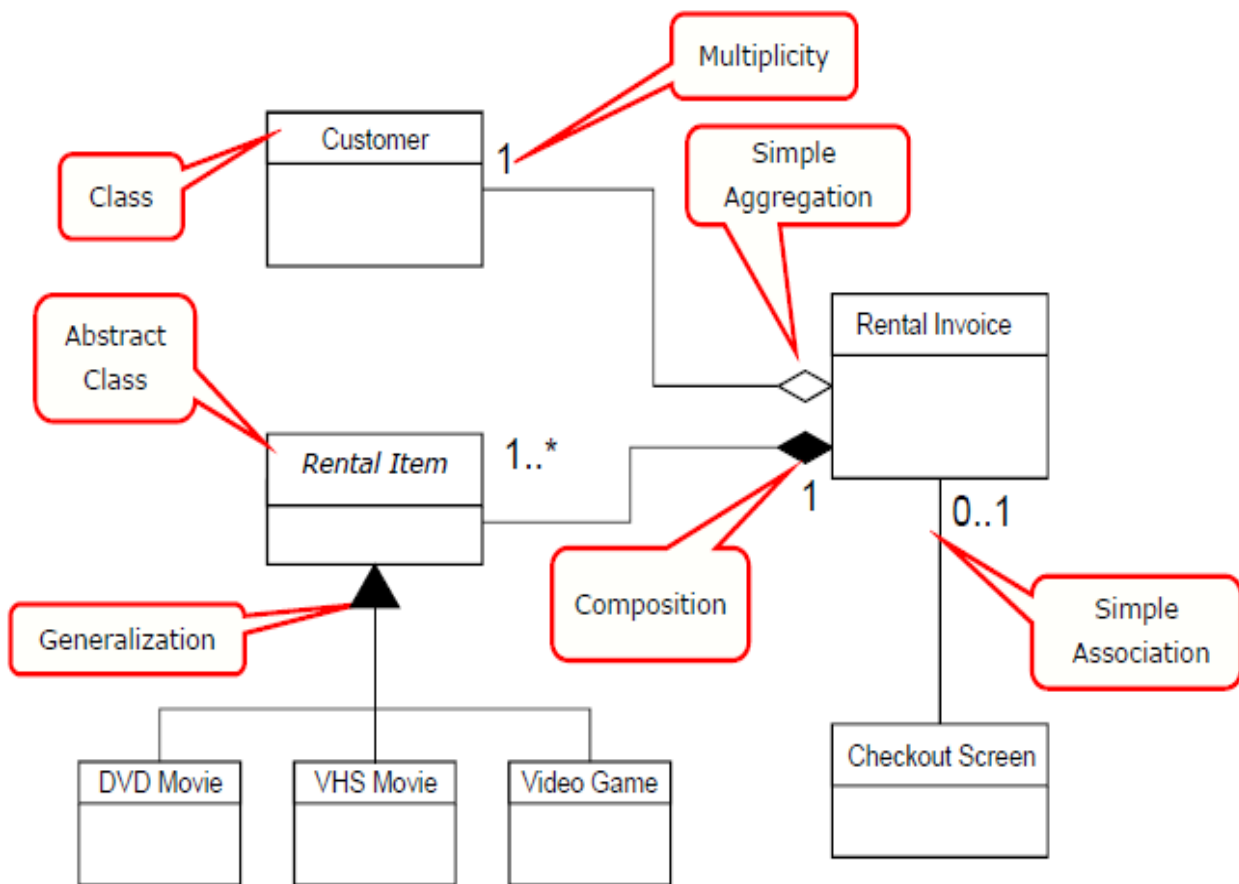
Figure: An Example of Class Diagram for “Video Rental System”
