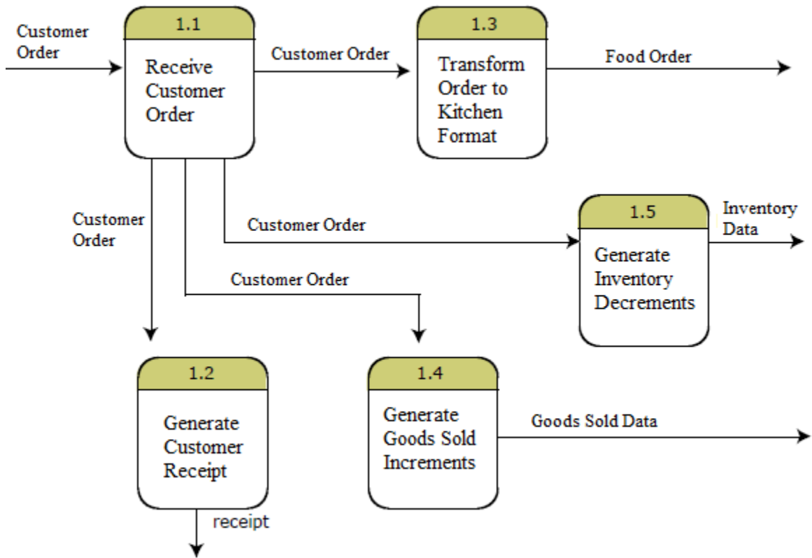
Figure: Level-1 Diagram Showing Decomposition of Process 1.0 from the Level-0 Diagram
