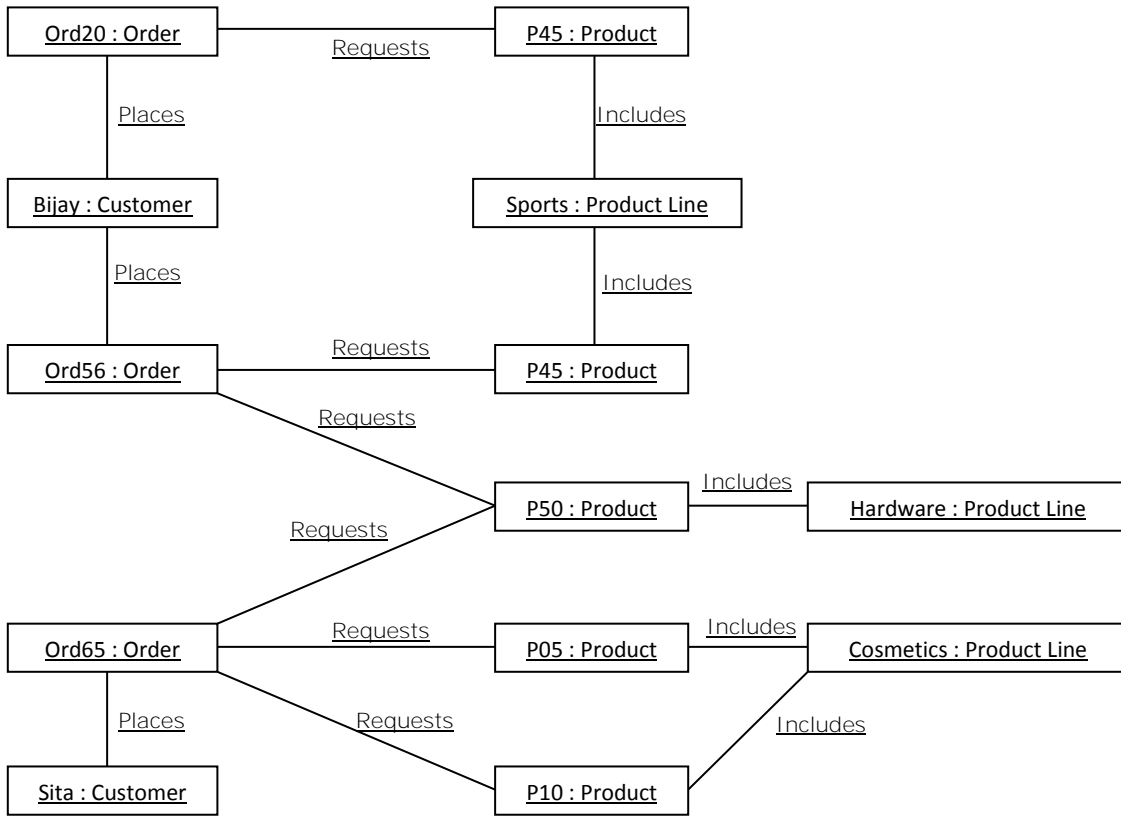
Figure: Object diagram for “Customer Order”
