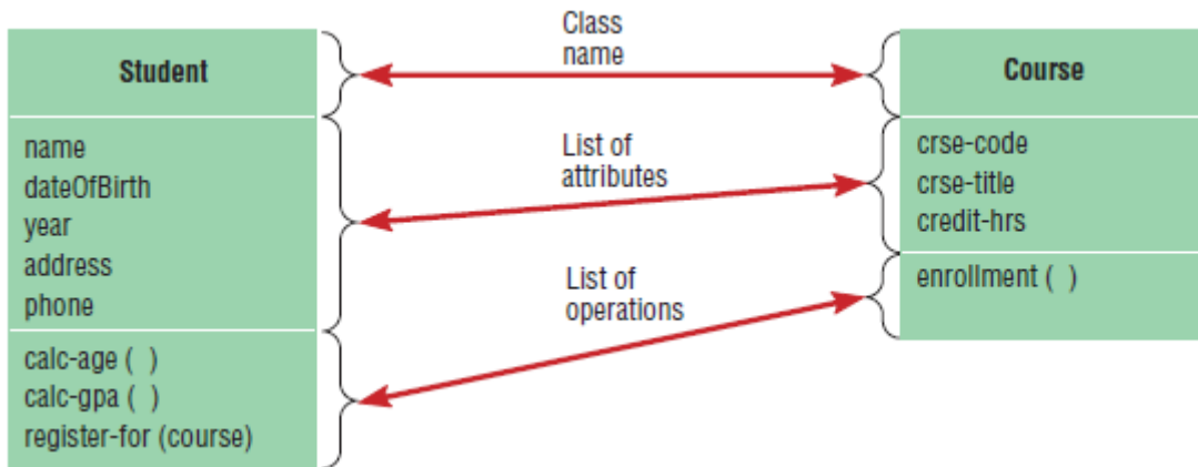
Figure: Class diagram showing two classes
