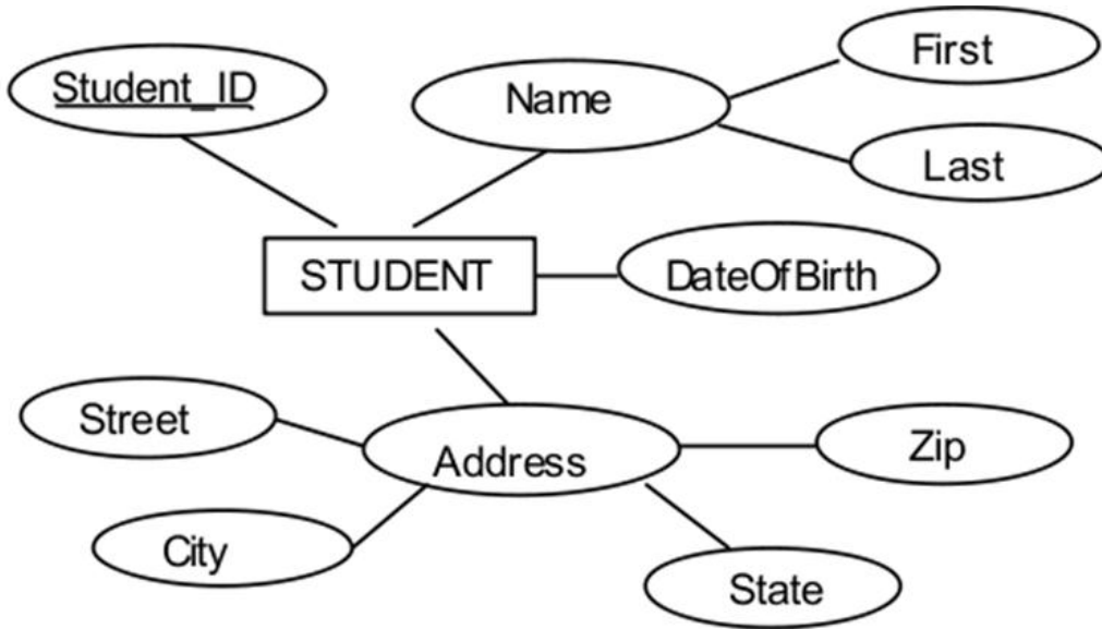
Figure: Example of composite attribute
