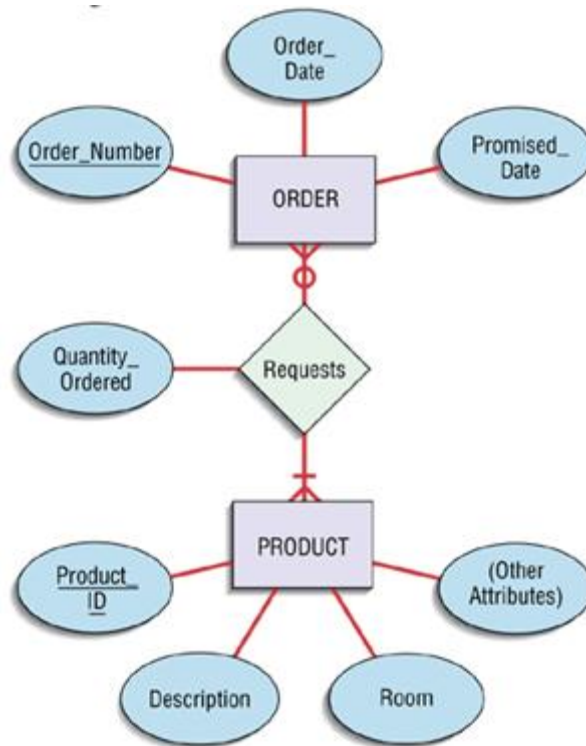
Figure: Representing a M:N relationship – ER Diagram
