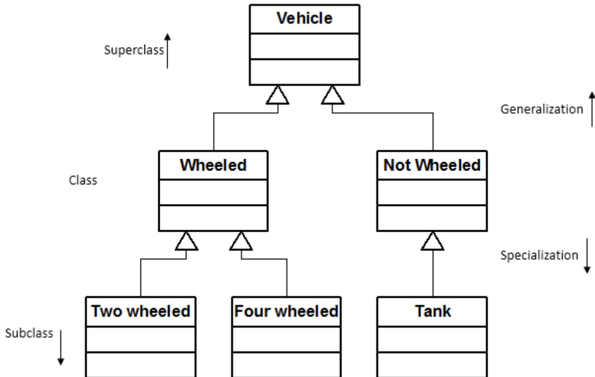
Figure: Example of Inheritance
