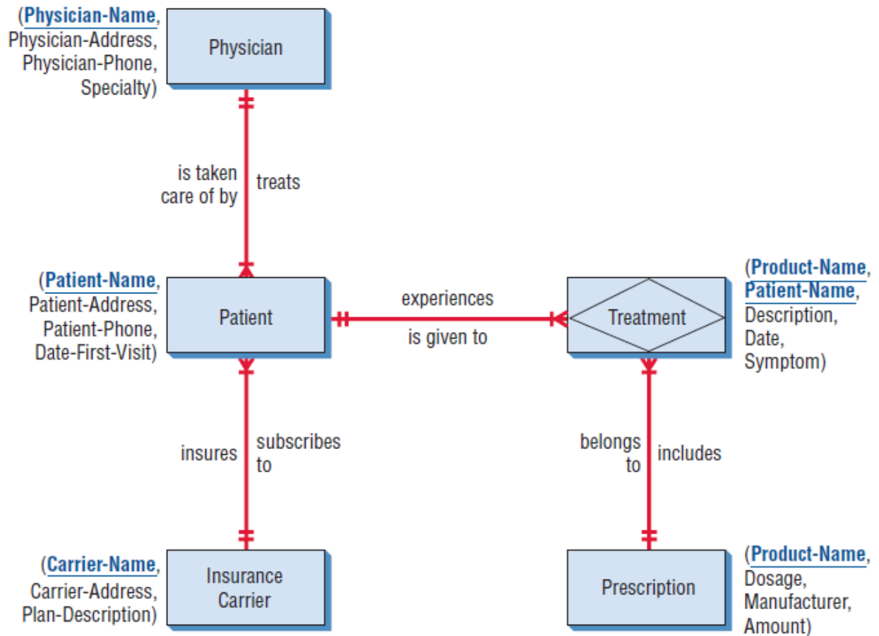
Figure: The entity-relationship diagram for patient treatment. Attributes can be listed alongside the entities. In each case, the key is underlined.
