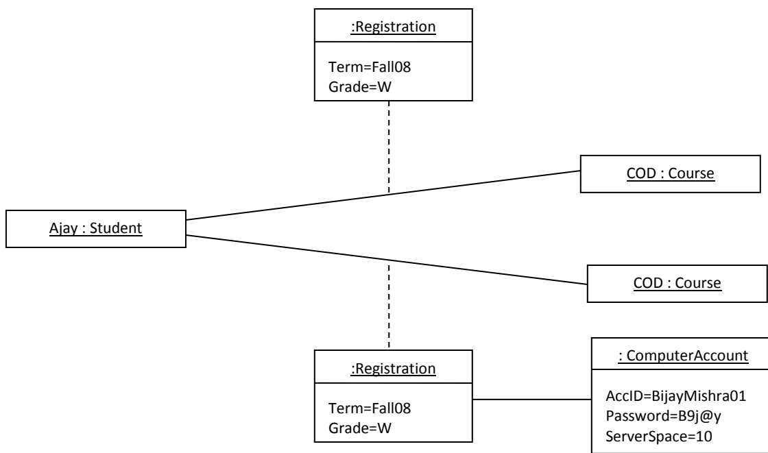
Figure: Object diagram for above class diagram
