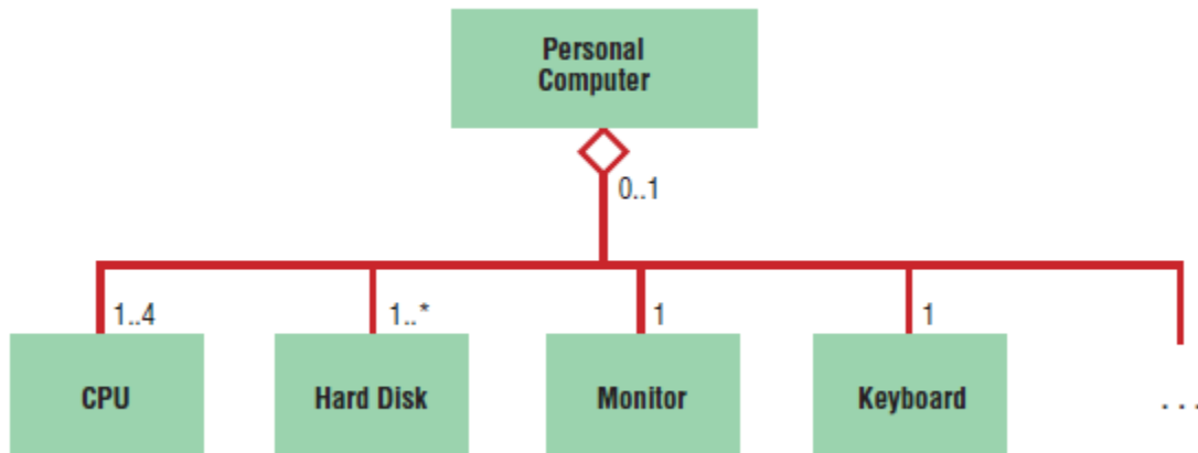
Figure: Example of aggregation.
