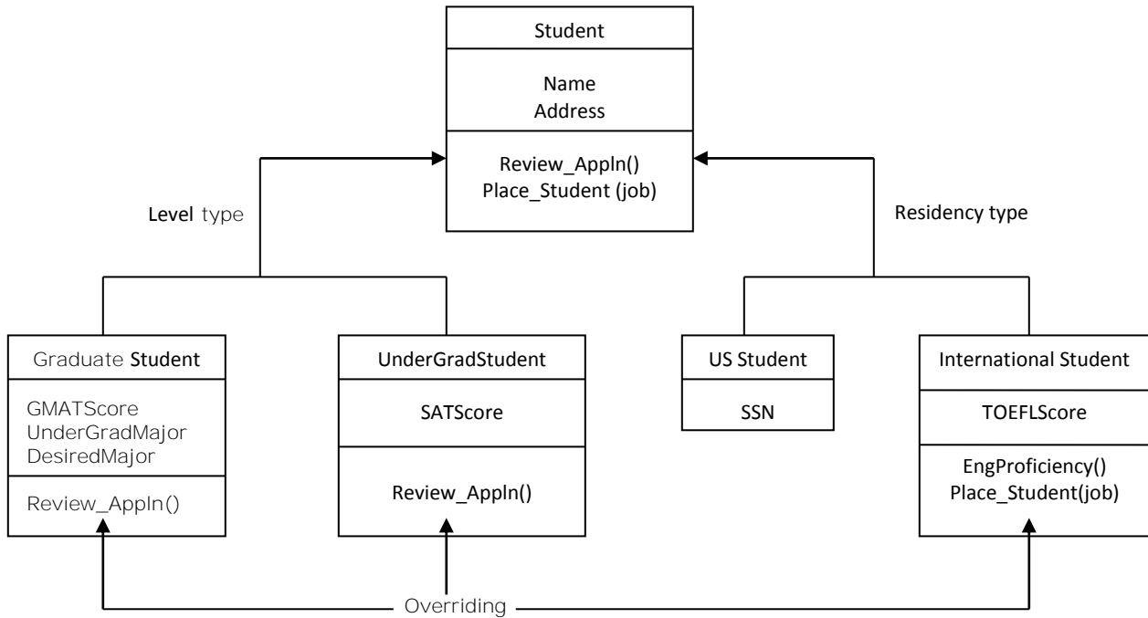
Figure: Overriding Inheritance
