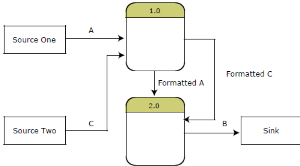
Figure: An unbalanced set of data flow diagrams – Figure A: Context Diagram and Figure B: Level-1 DFD
