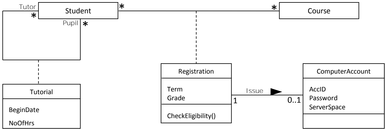
Figure: Class diagram showing two association classes
