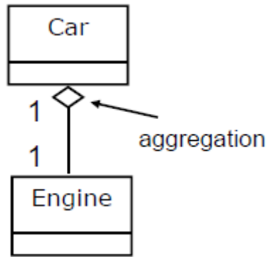
Example: Aggregation Example
